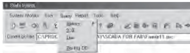
Fig. 7-1 Data Query
